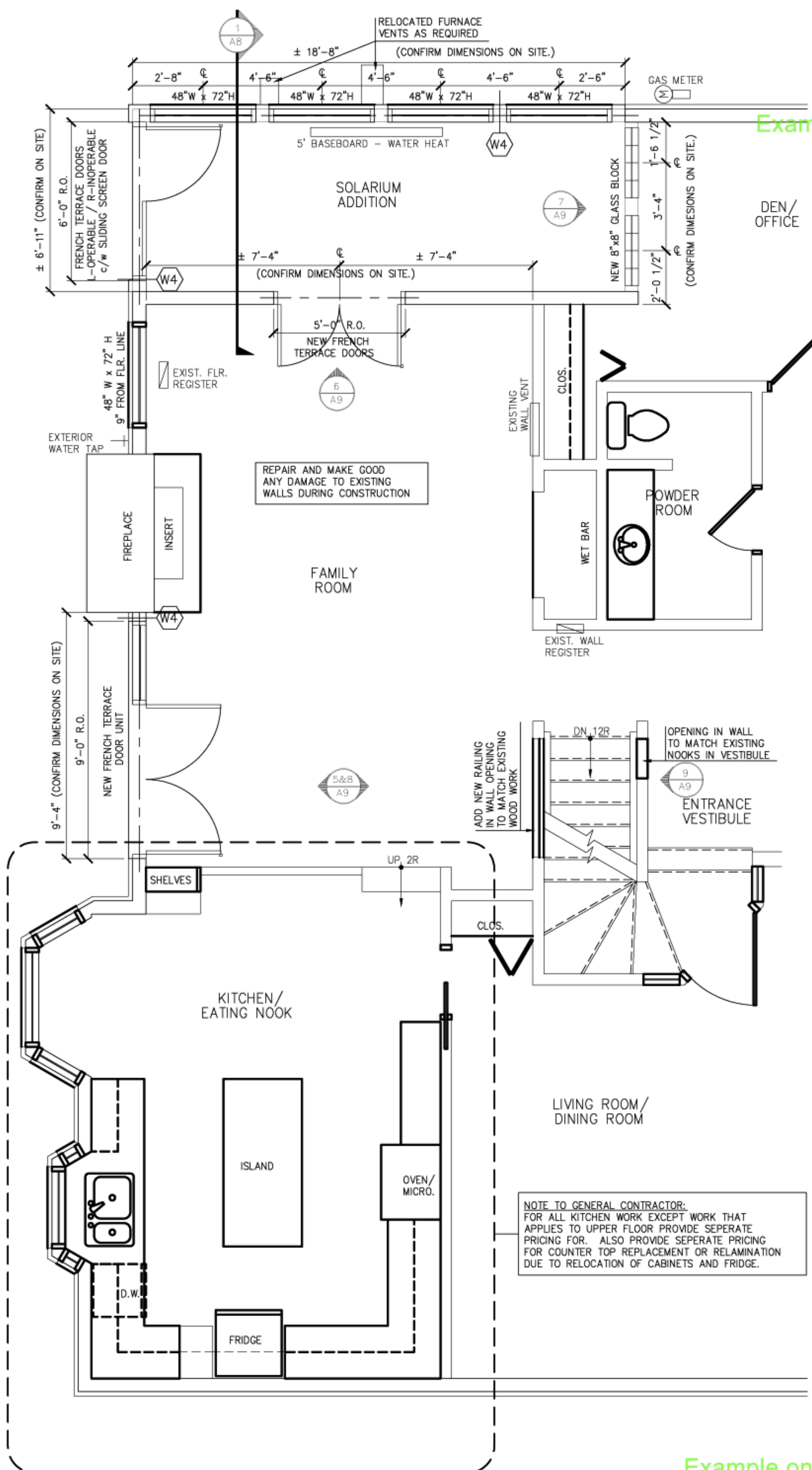
2 A3 MAIN FLOOR RENOVATION PLAN SCALE: 3/8" = 1'-0"
