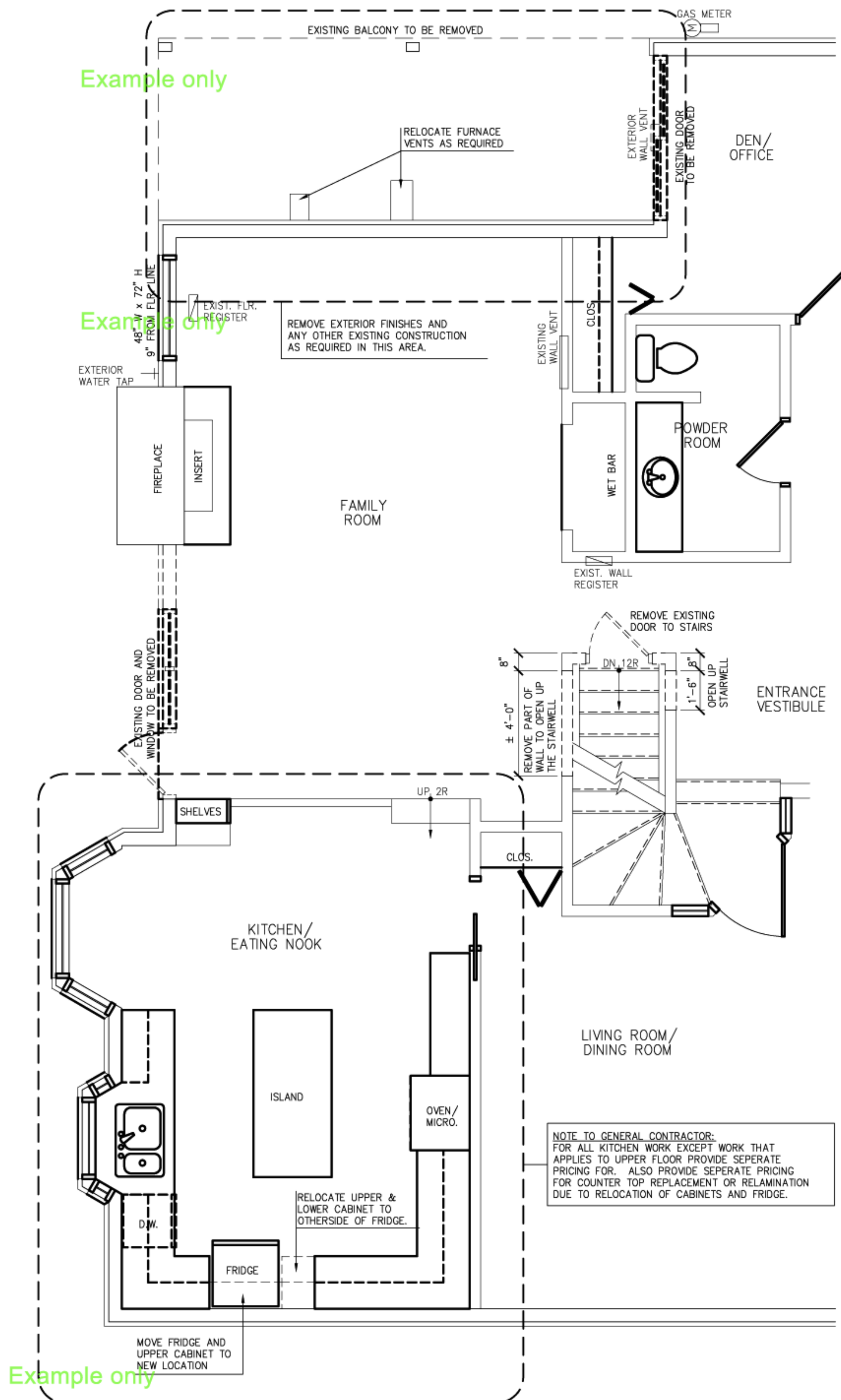
1 A3 MAIN FLOOR DEMOLITION PLAN SCALE: 3/8" = 1'-0"
